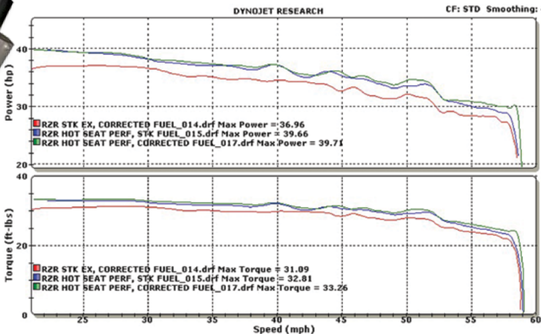
Hot Seat Performance - Corrected Fuel Gains
